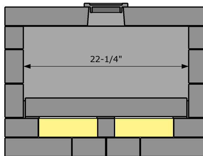
Section - Front
