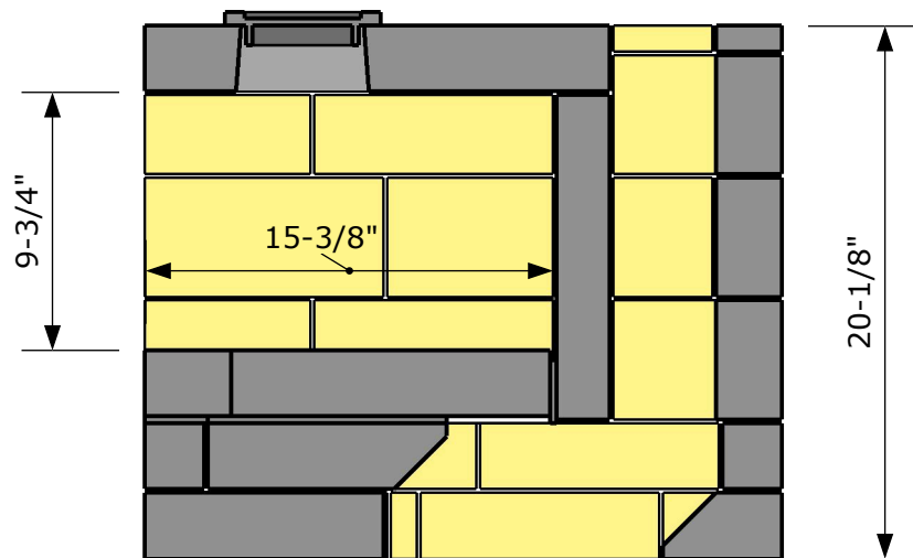
Section - Side
