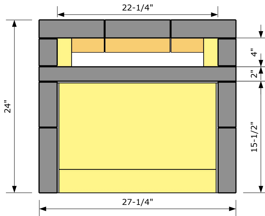
Section - Top
